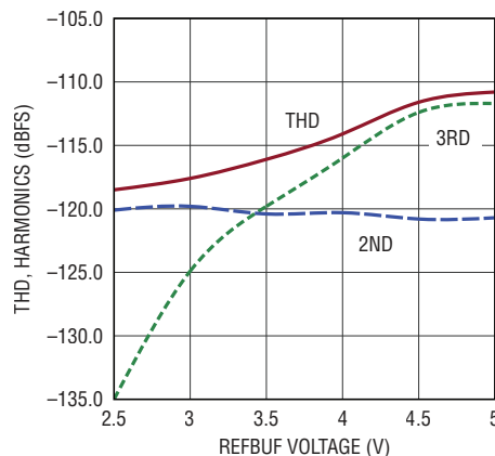
THD, Harmonics vs \text{REF}_{BUF} , f_{IN} = 1\text{kHz}
