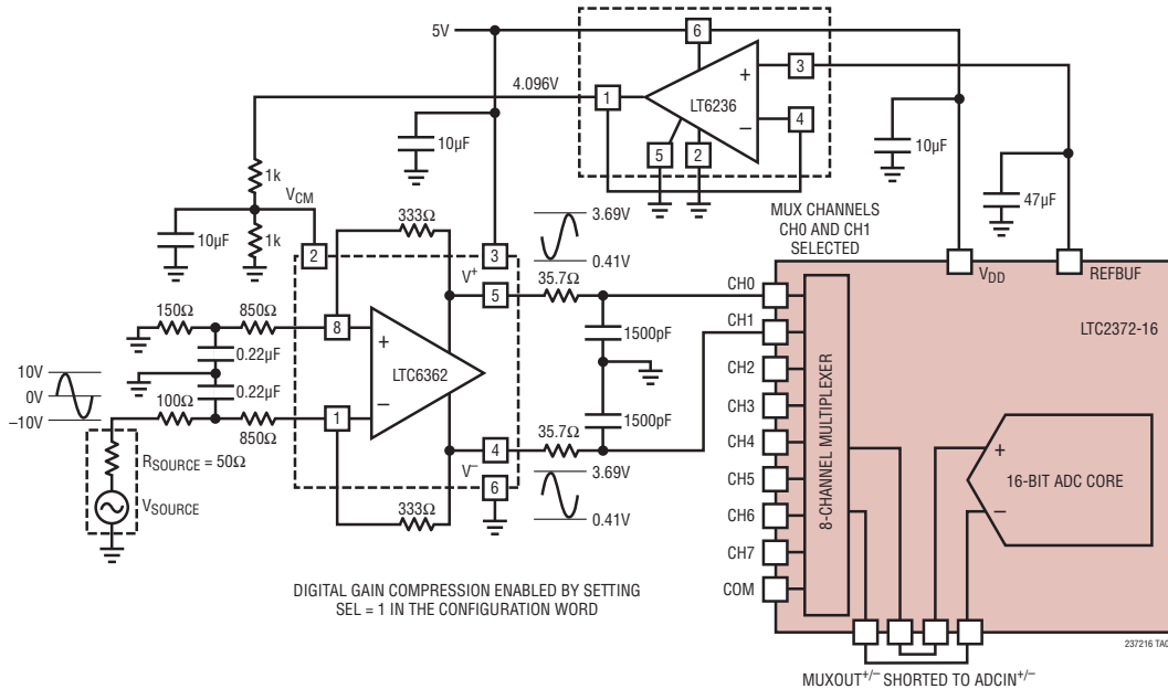
LTC6362 Configured to Accept a \pm 10\text{V} Input Signal Using a Single 5V Supply with Digital Gain Compression Enabled on the LTC2372-16
